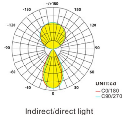
Photometric Diagram
